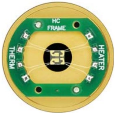
Heat Capacity
